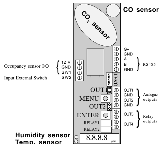
PCB & terminals of model mSENSE II
